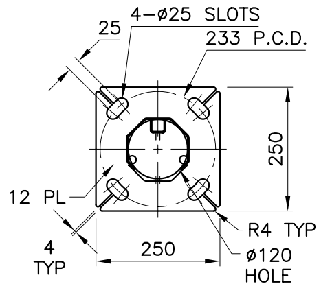
BASEPLATE DETAIL
