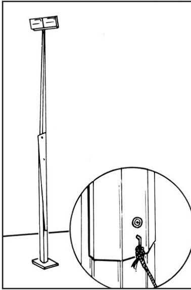
Figure 3. Raising and Lowering of Seesaw Columns
