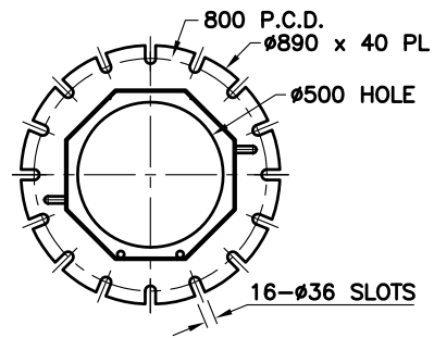
BASEPLATE DETAIL 1:20
