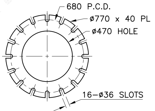
VIEW A SCALE 1:20 BASEPLATE FOR 16- M30 RAGBOLTS
