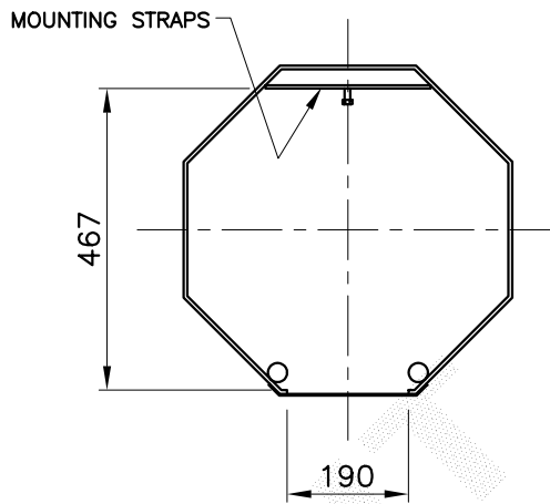
CONTROL GEAR CLEARANCES 1:10
