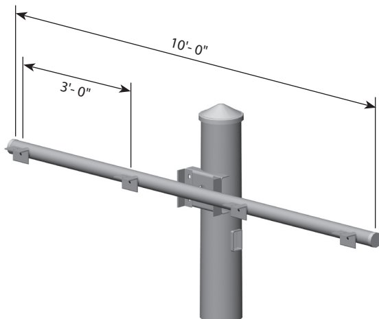
CR 4 (4 Fixtures)
