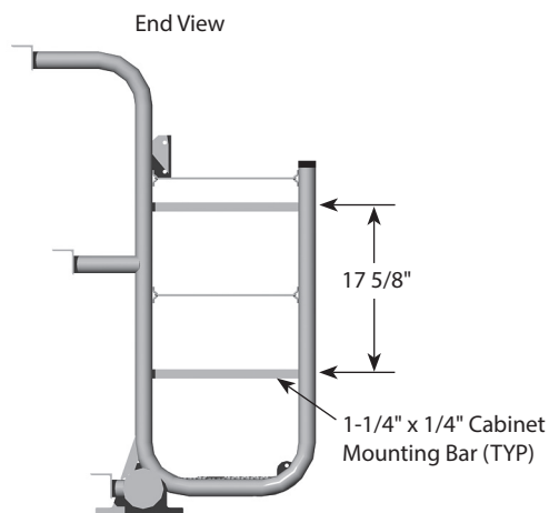
CONTROL PANEL - CAGE MOUNT
