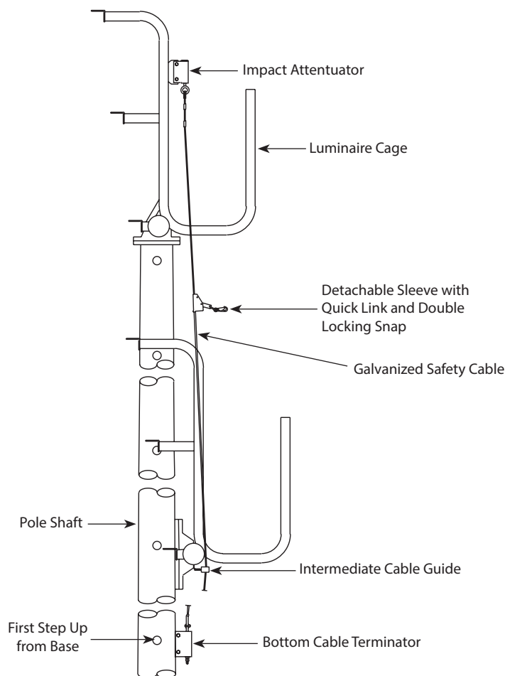
SAFETY CABLE CLIMBING DEVICE
