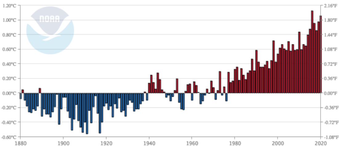
Global Land and Ocean March–May Temperature Anomalies
