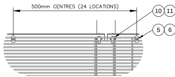
DETAIL A
