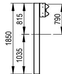
SECTION B-B 1850mm C-Post w/ 360mm C-Block
