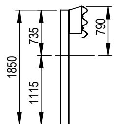
SECTION F-F 1850mm C-Post w/ RHS Block
