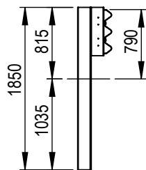
SECTION E-E 1850mm C-Post w/ 550mm C-Block
