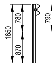
SECTION A-A Ezy-Guard 4 Post
