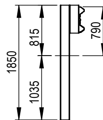
SECTION D-D 1850mm C-Post w/ 450mm C-Block
