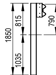
SECTION C-C 1850mm C-Post w/ 360mm C-Block
