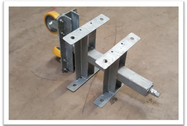
Wheel Set
