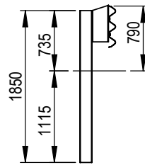
SECTION F-F 1850mm C-Post w/ RHS Block
