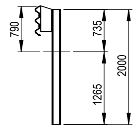
SECTION F-F 2000mm C-Post w/ RHS Block
