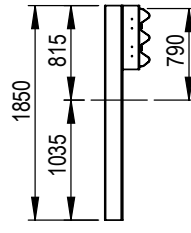
SECTION E-E 1850mm C-Post w/ 550mm C-Block
