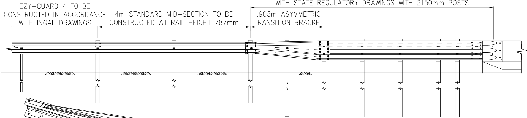
ELEVATION VIEW
