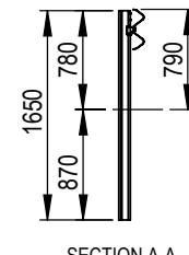
SECTION A-A Ezy-Guard 4 Post
