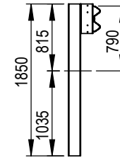
SECTION C-C 1850mm C-Post w/ 360mm C-Block
