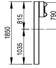
SECTION D-D 1850mm C-Post w/ 450mm C-Block
