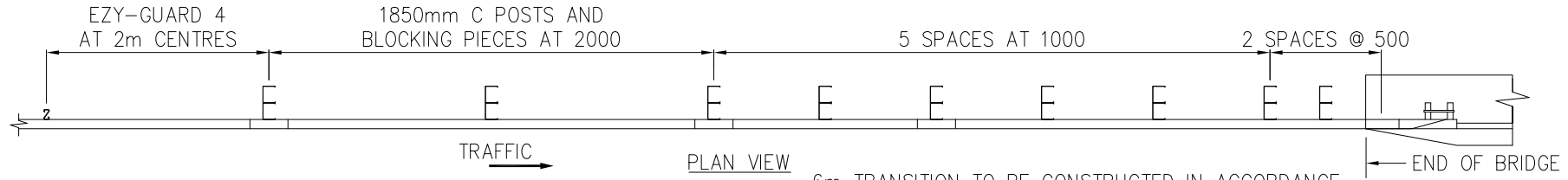
VICROADS TYPE-B 10m BRIDGE APPROACH
