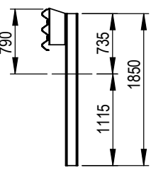
SECTION E-E 1850mm C-Post w/ RHS Block
