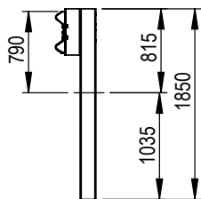
SECTION C-C 1850mm C-Post w/ 450mm C-Block
