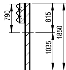
SECTION D-D 1850mm C-Post w/ 550mm C-Block
