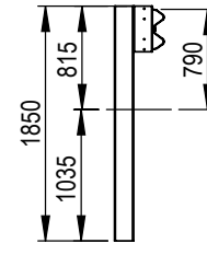
SECTION B-B 1850mm C-Post w/ 360mm C-Block
