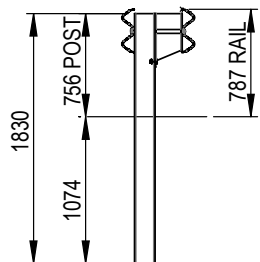
SECTION C-C SCALE 1 : 50
