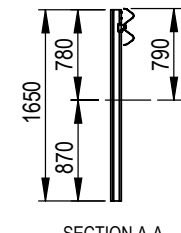
SECTION A-A Ezy-Guard 4 Post
