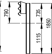
SECTION E-E 1850mm C-Post w/ RHS Block
