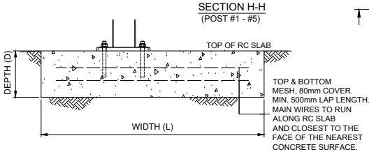
TYPICAL 9.5M LONG RC SLAB SECTION-REINFORCING MESH OPTION
