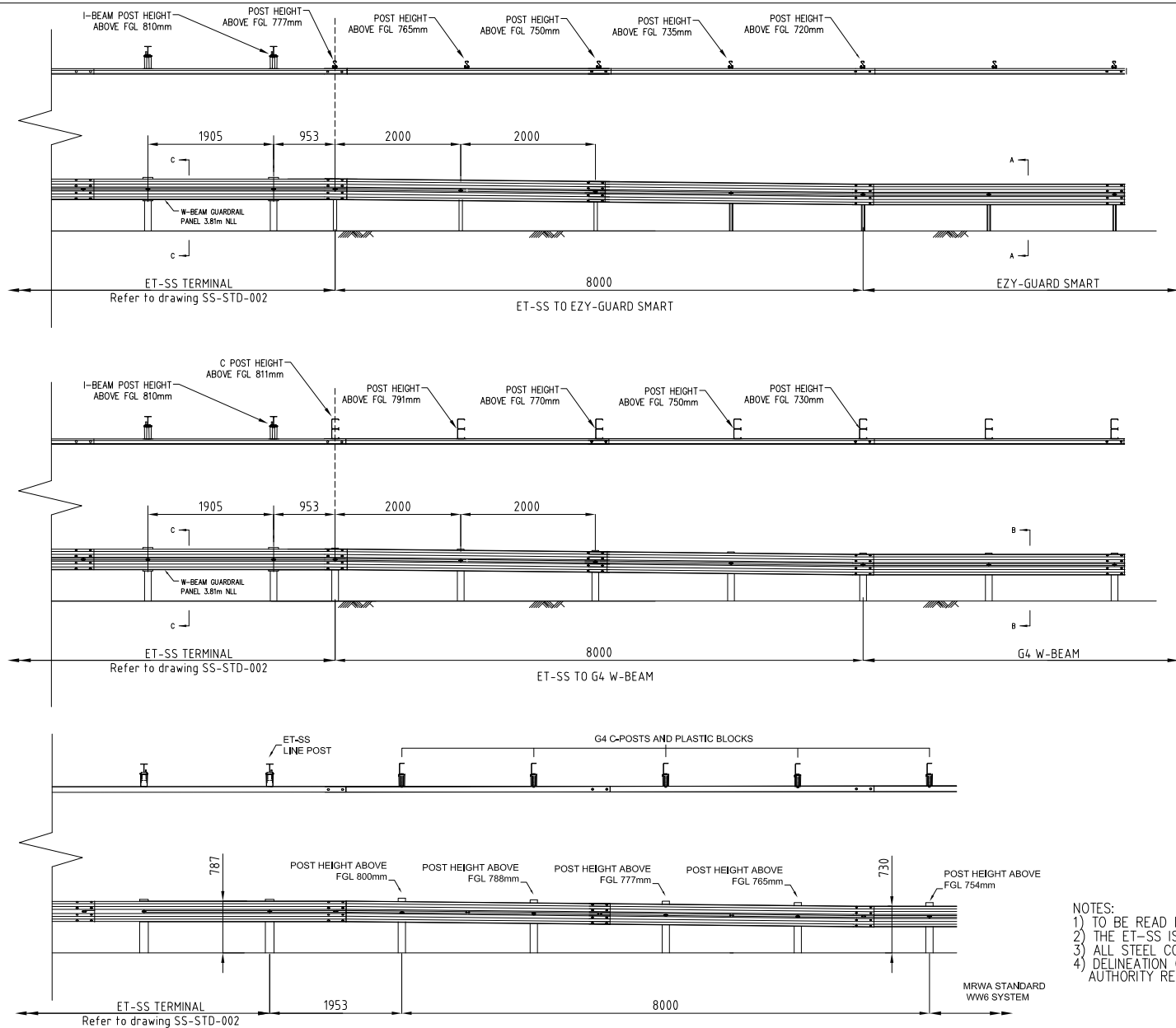
SECTION "A-A"
