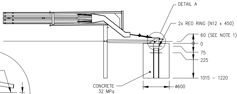
OPTION 03 – Ø600 PIER FOUNDATION
