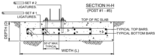
TYPICAL 9.5M LONG RC SLAB SECTION-REINFORCING BAR OPTION
