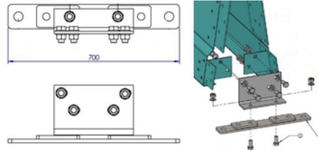
BG800 Intermediate Anchor Bolted Joint Assy (BG-50-07)
