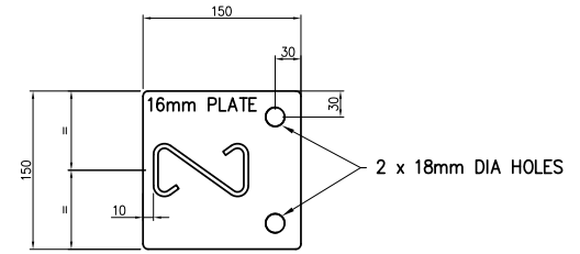
Z-POST ON BASE PLATE PLAN VIEW
