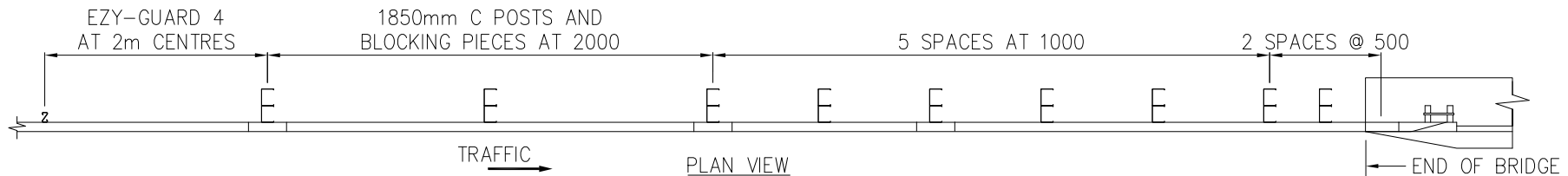
PLAN VIEW
