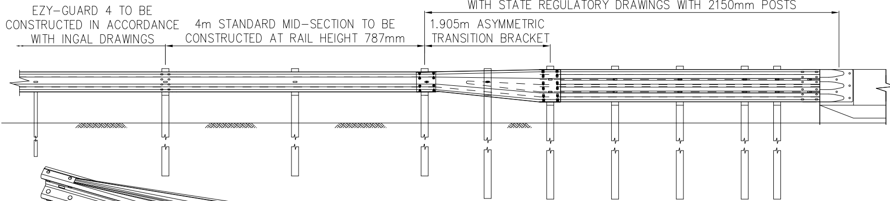
ELEVATION VIEW
