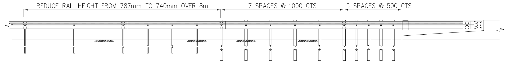
VICROADS TYPE-B 10m BRIDGE APPROACH
