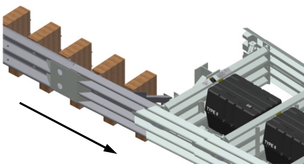
Figure 46 Quad-Beam™ to Thrie-Beam
