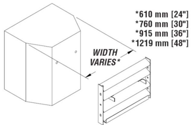
Figure 8 Concrete Backup
