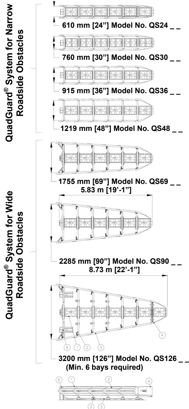
Figure 1 Plans & Elevation
