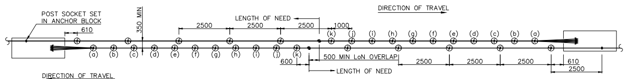
INTERMEDIATE ANCHOR GENERAL ARRANGEMENT (DIMENSIONS INDICATIVE OF 2.5m BARRIER POST SPACING)
