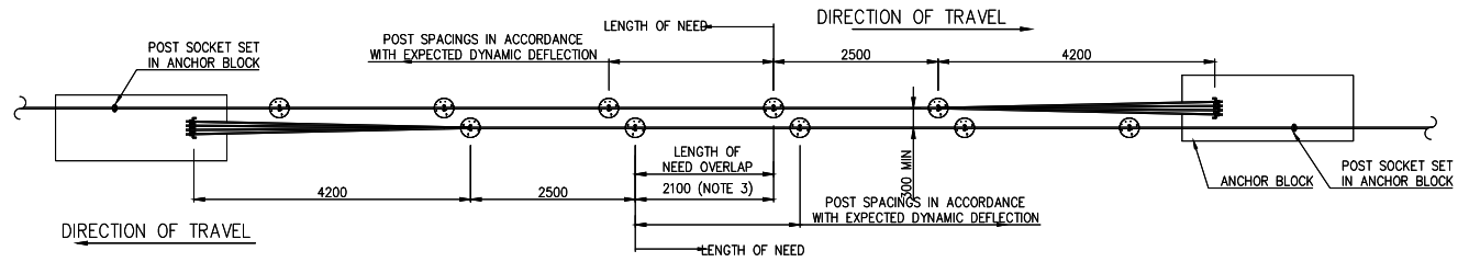
INTERMEDIATE ANCHOR GENERAL ARRANGEMENT
