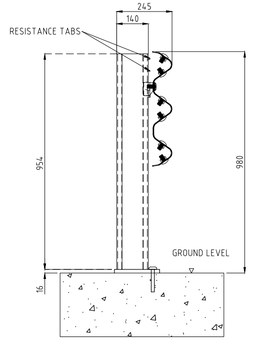
HC "Z" POST & CARRIAGE ASSEMBLY SIDE VIEW
