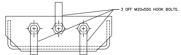
SECTION B NTS
