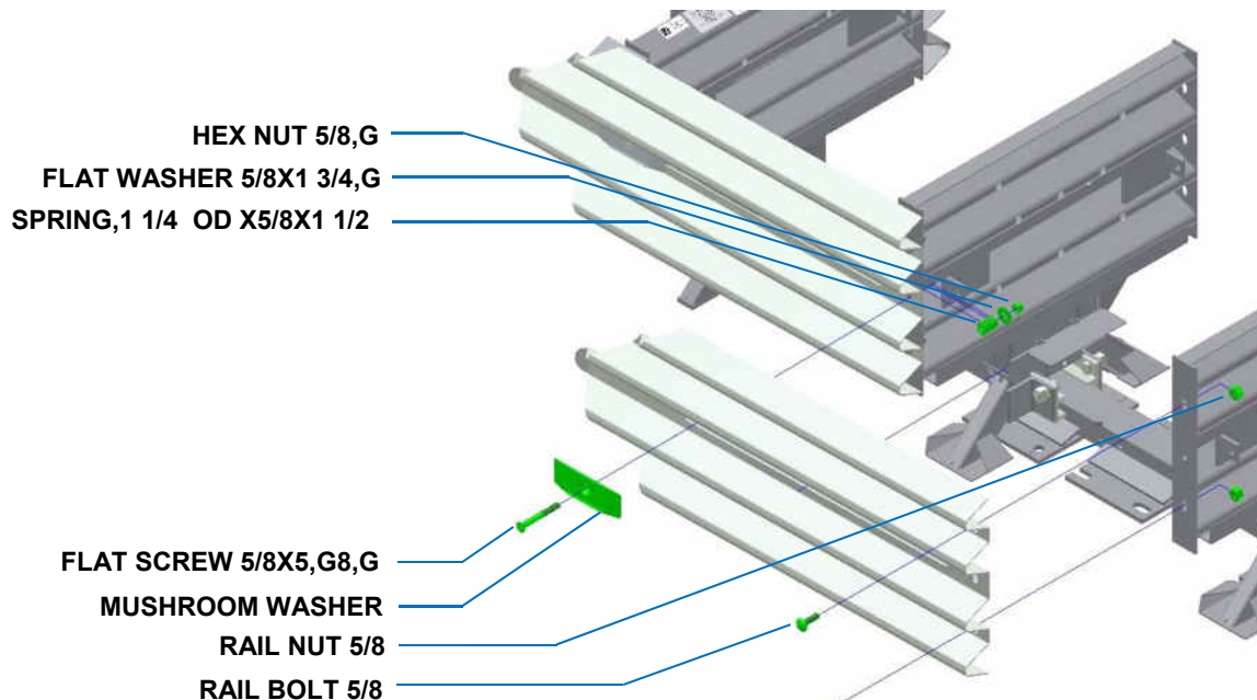
Figure 22 Fender Panel Assembly
