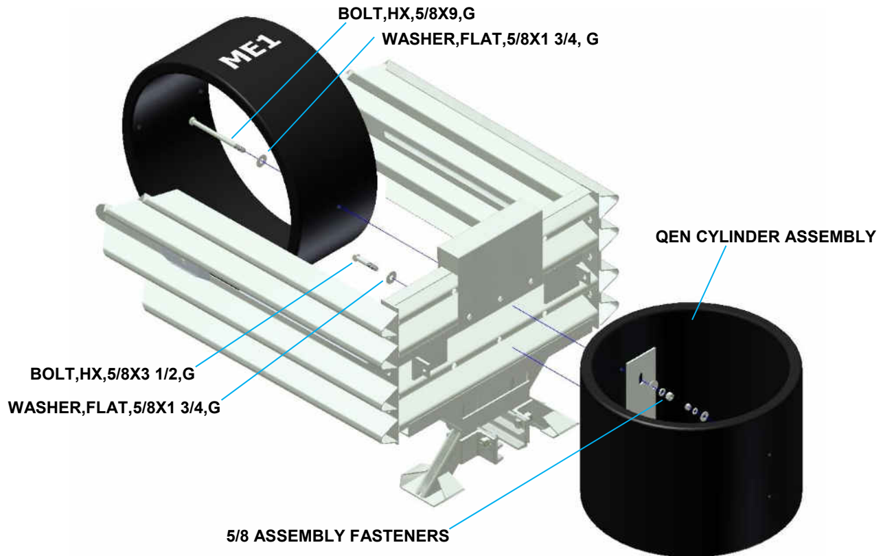
Figure 28 Attach Nose Cylinder to First Diaphragm
