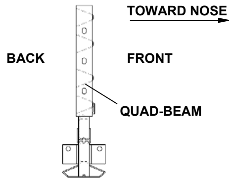
Figure 18 Diaphragm Orientation
