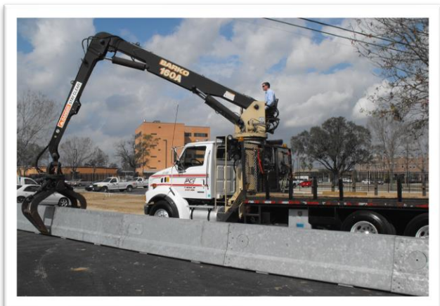
Lifting Grab
