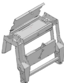
BG800 Lifting Cradle
