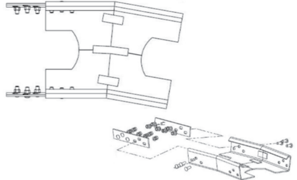
10 Deg T-Top Assembly
