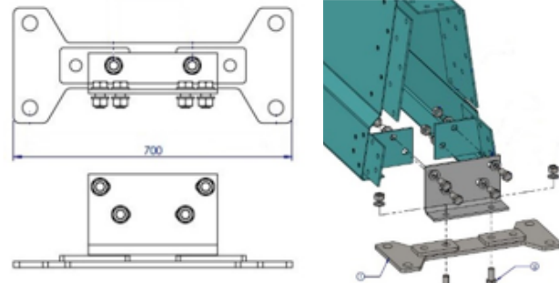
BG800 Bow Tie Anchor Bolted Joint Assy (BG-50-08)
