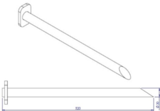
Flat Top Pin
