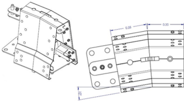
10 Deg LH Bolted QuickLinks
