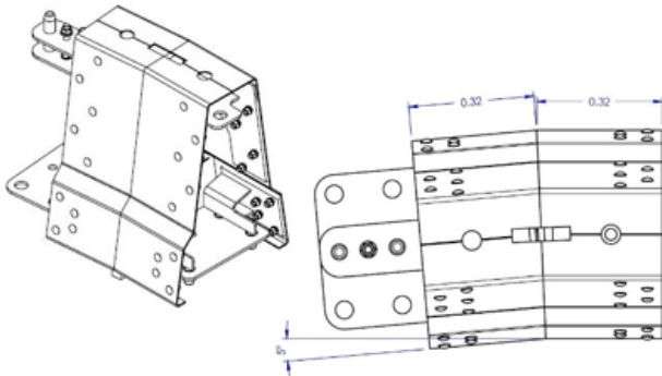
5 Deg LH Bolted QuickLinks
