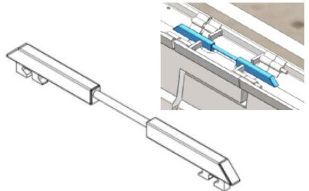
T-Top Turn Buckle Assy - Galv
