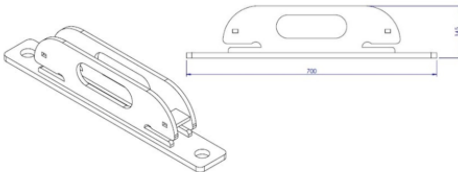
BG800 Clamp-in Intermediate Anchor Assy
