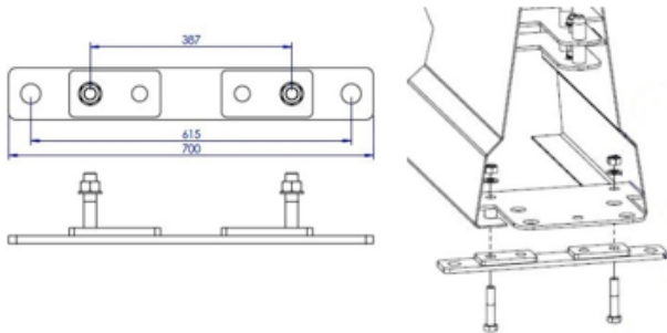
BG800 Intermediate Anchor Assy (BG-50-09)
