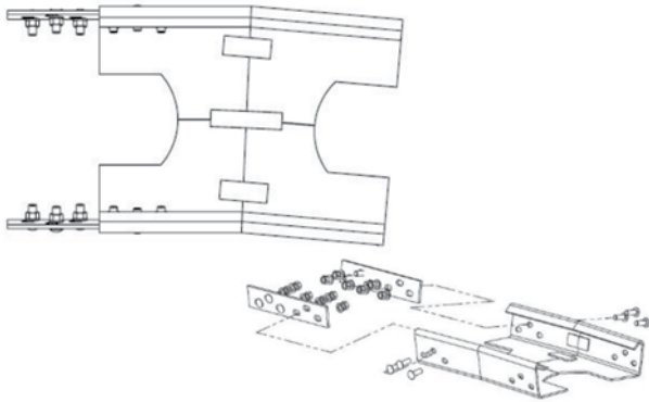
5 Deg T-Top Assembly
