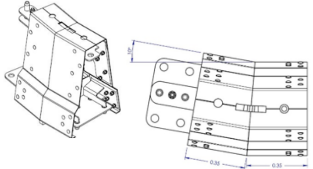
10 Deg RH Bolted QuickLinks
