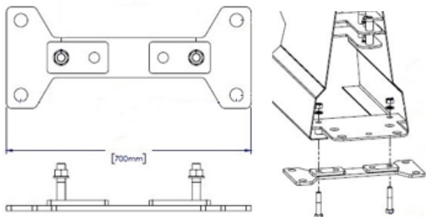
BG800 Bow Tie Anchor Assy (BG-50-10)
