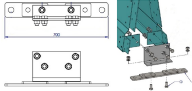
BG800 Intermediate Anchor Bolted Joint Assy (BG-50-07)
