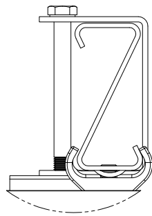
DETAIL C
