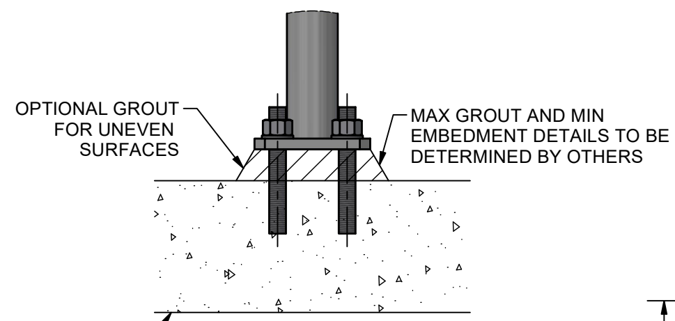
DETAIL 1 FOOTING DETAIL FOR CONCRETE MOUNTING
