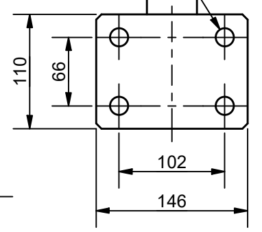
DETAIL 3
