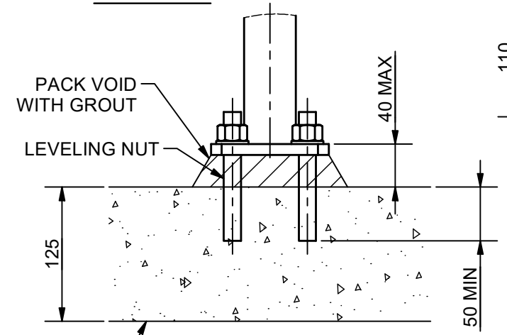
DETAIL 1
