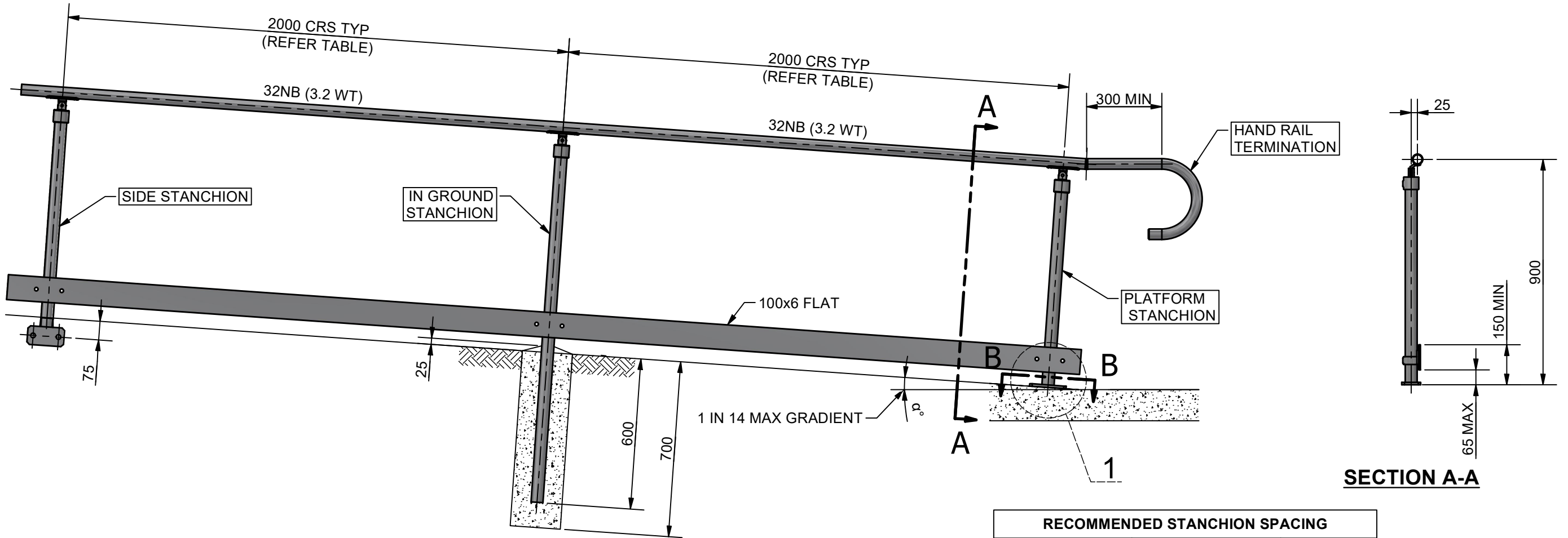
ELEVATION VIEW
