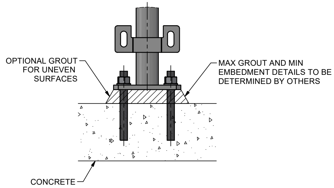
DETAIL 1 FOOTING DETAIL FOR CONCRETE MOUNTING KERB RAIL NOT SHOWN FOR CLARITY
