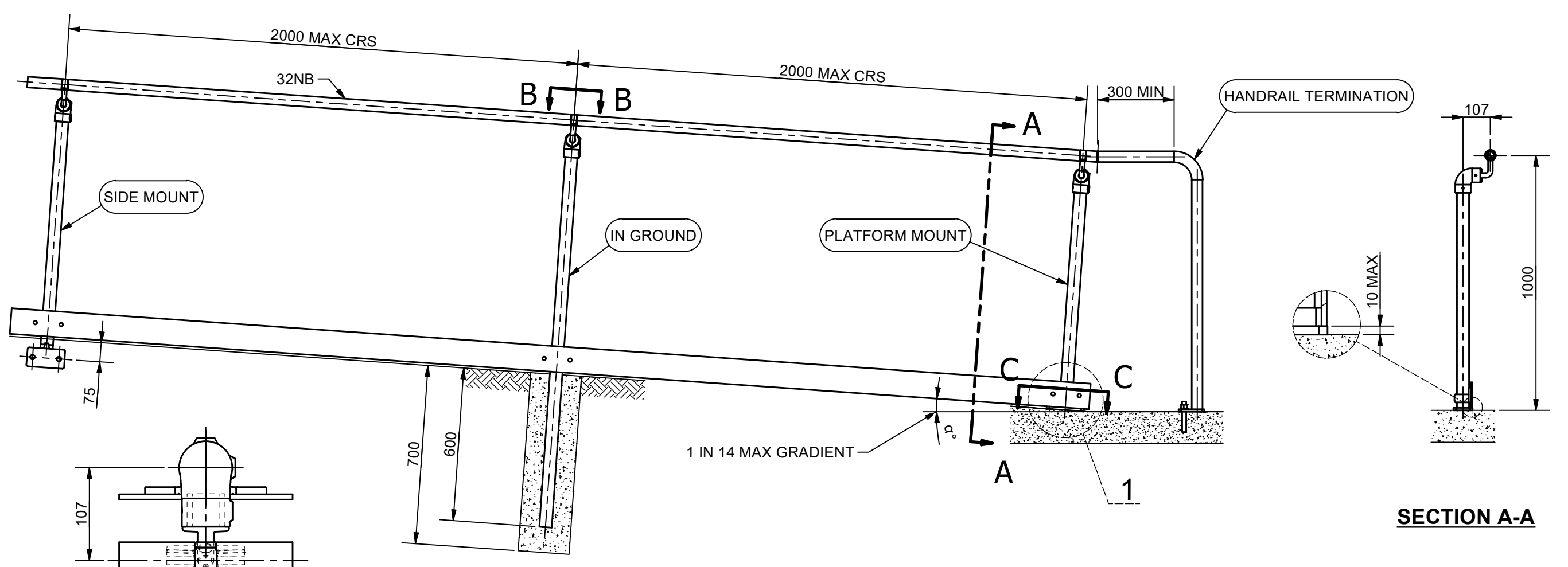
ELEVATION VIEW
