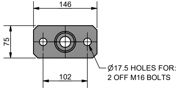
SECTION B-B TYPICAL BASE PLATE DETAIL FOR PLATFORM AND SIDE STANCHIONS
