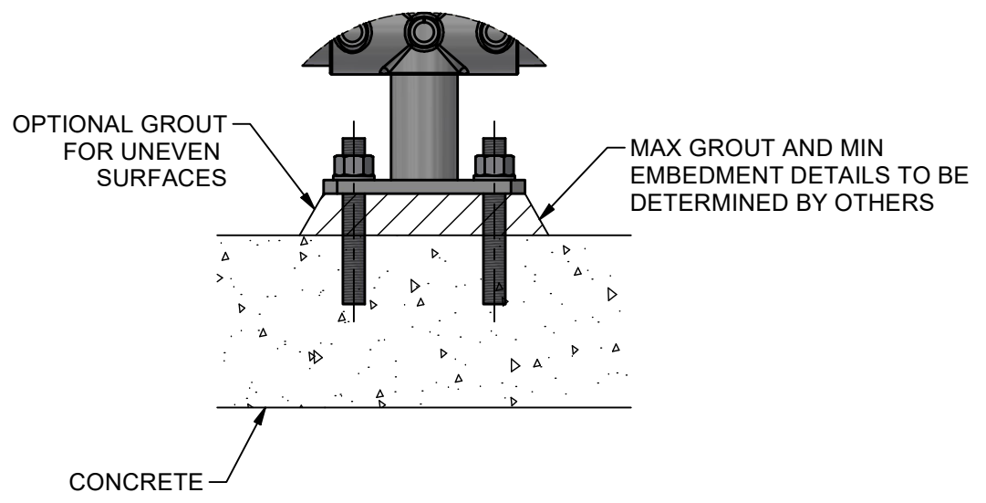
DETAIL 2 FOOTING DETAIL FOR CONCRETE MOUNTING
