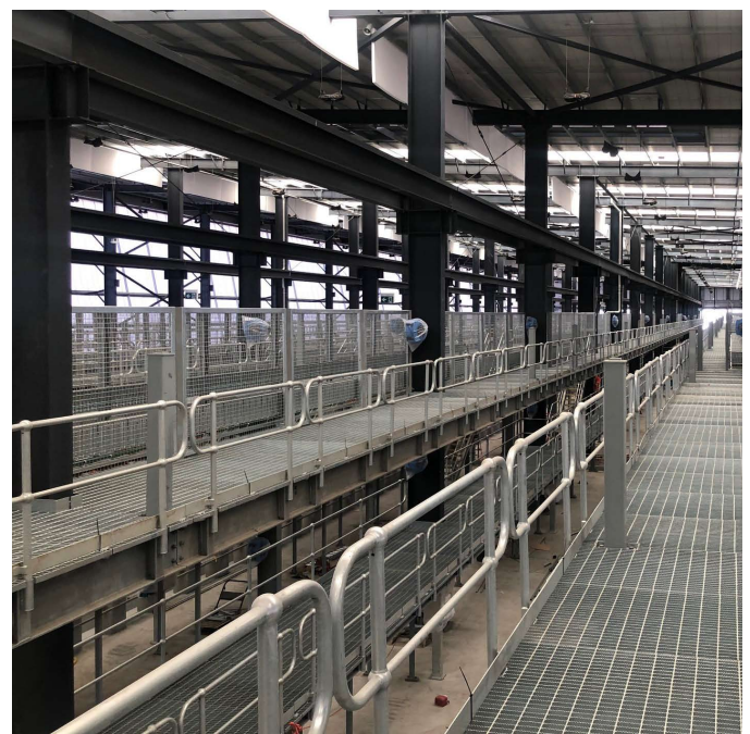
Rail Maintenance Walkways for Bridge Structures
