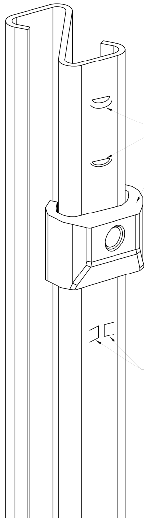
Z-POST & CARRIAGE ASSEMBLY ISOMETRIC VIEW
