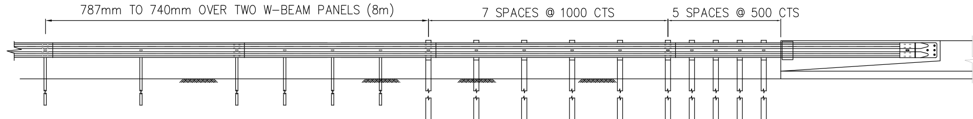
VICROADS TYPE-B 10m BRIDGE APPROACH
