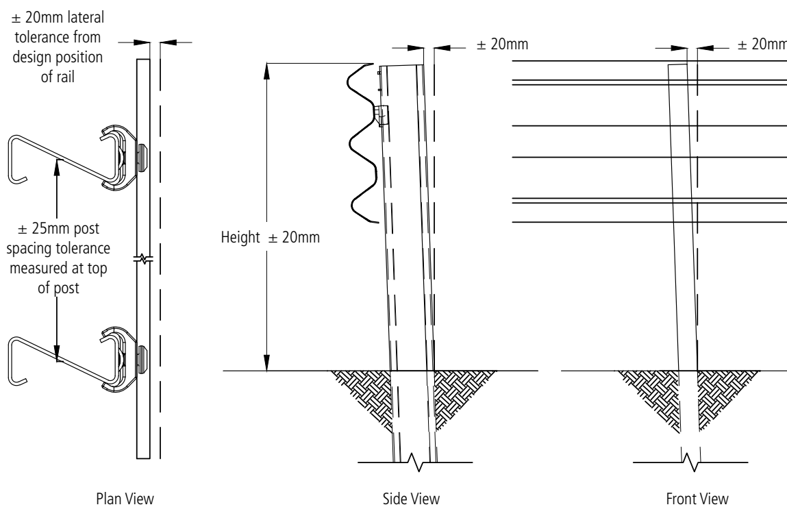
Figure 16: Ezy-Guard HC Installation Tolerances
