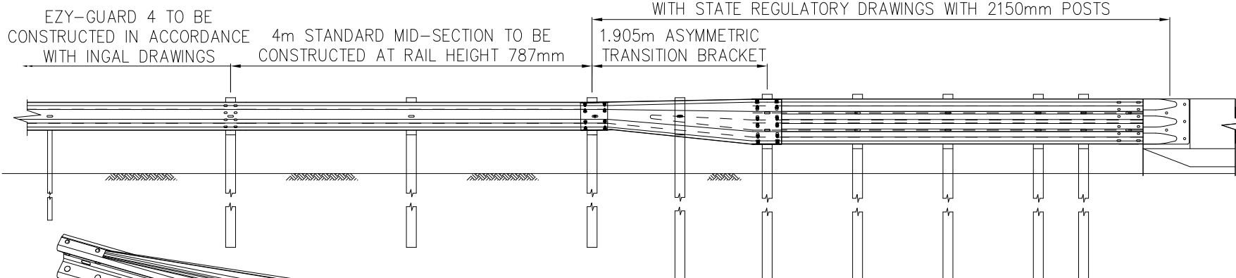
ASYMMETRIC TRANSITION BRACKET
