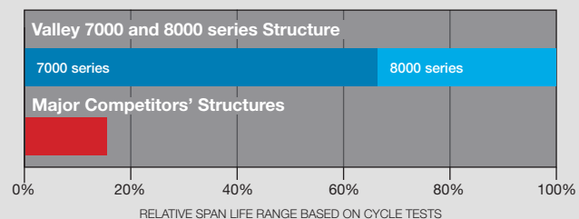
Accelerated Structural Life Cycle Test Comparison
