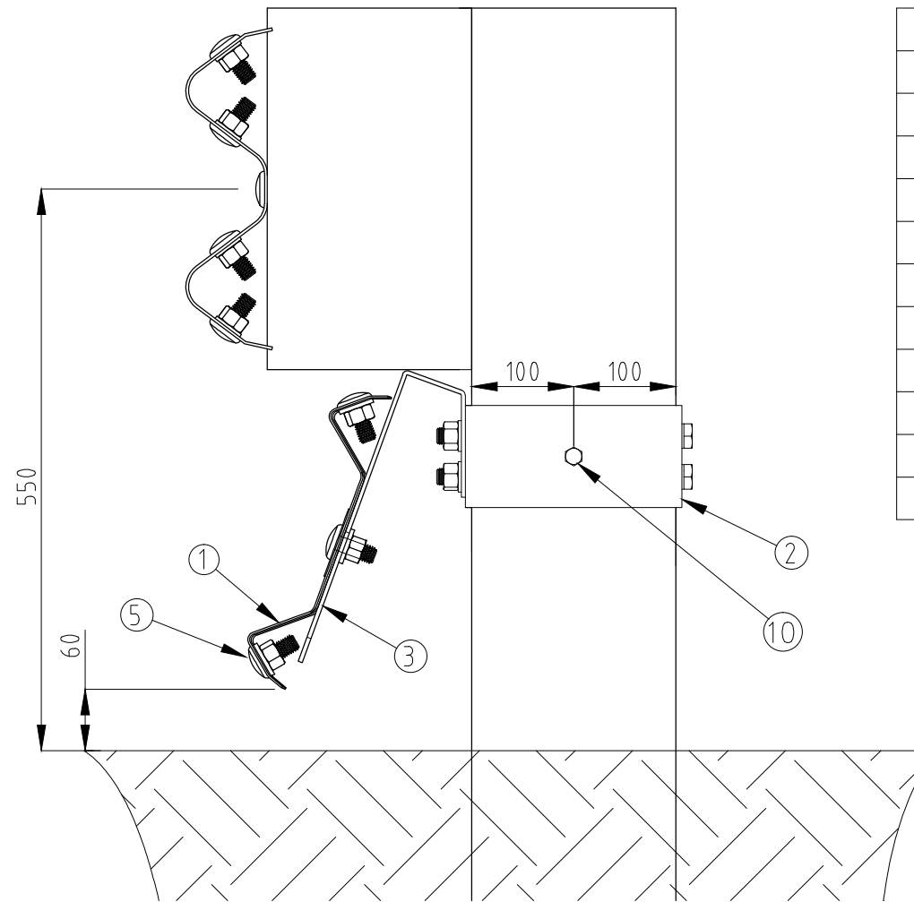
DEPARTURE-SIDE ELEVATION VIEW
