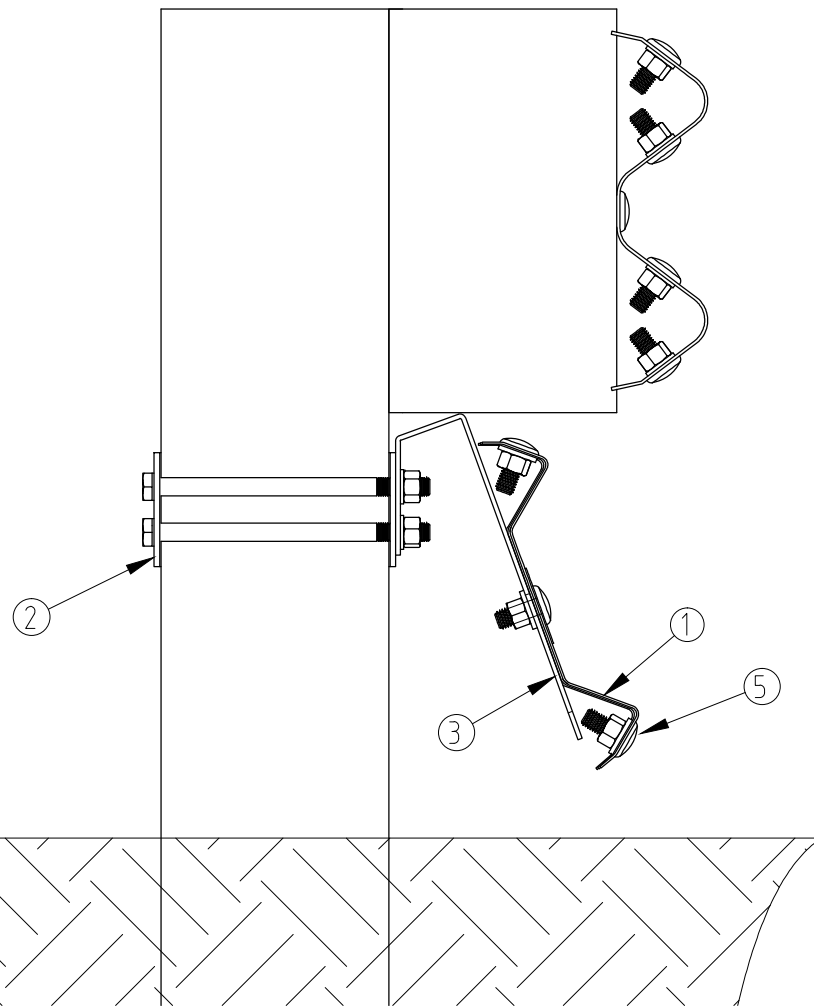
APPROACH-SIDE ELEVATION VIEW
