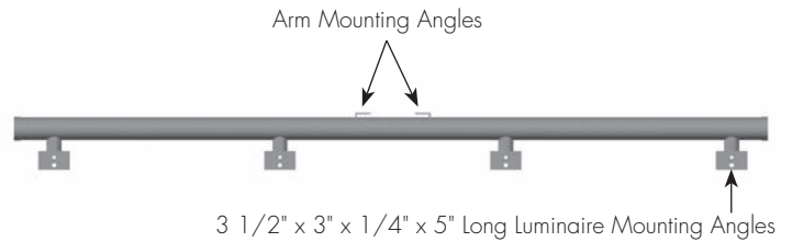
CROSSARM DETAIL TOP VIEW
