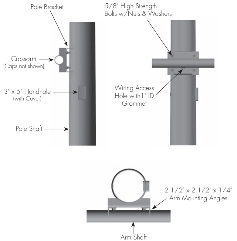
CROSSARM MOUNTING DETAILS
